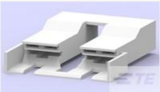
TE Part #1-521253-7 FASTON PL 250 HSG REC BLUE NYLON 66/6
