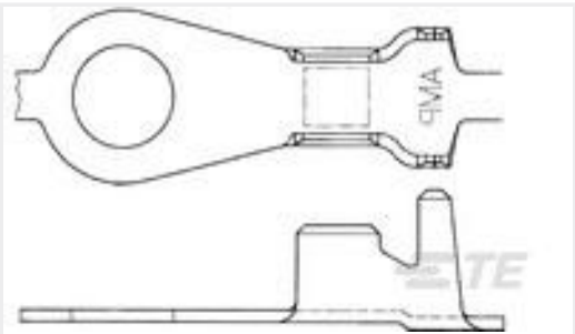
TE Part #881001-2 RING TONGUE 6.0-10.0 MM2 1.00X21.7 TPBR
