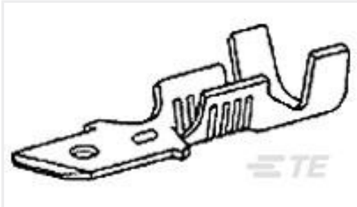
TE Part #350969-1 MR GRND PIN 26-18 PTPPHBZ
