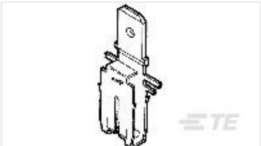
TE Part #63464-3 MAG-MATE 250 F-TAB TPBR
