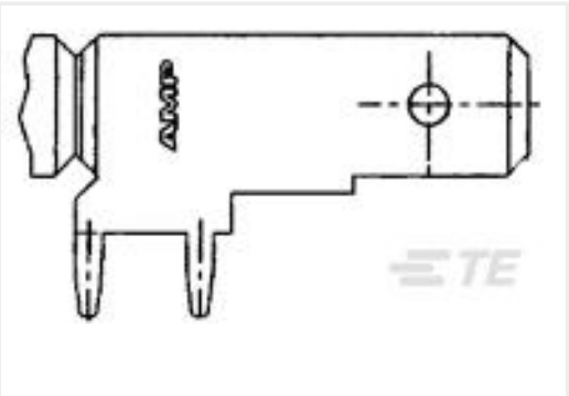
TE Part #63952-1 250 FASTON TAB TPBR
