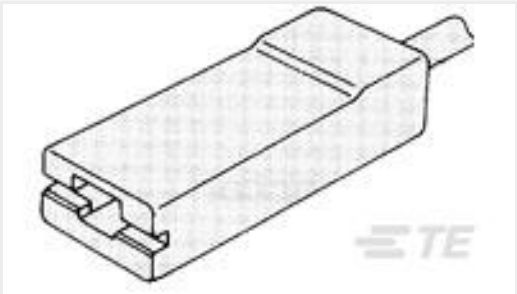
TE Part #179974-1 250 PL EX REC. 18-14AWG TPBR
