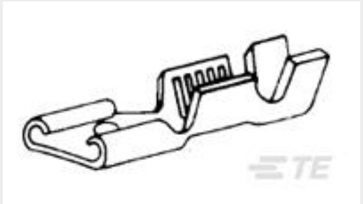
TE Part #60385-2 .250 FAST REC IS 18-2/17 TPBR
