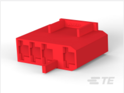
TE Part #2-521498-2 250 FASTON HSG.,REC.,4 POS,RED
