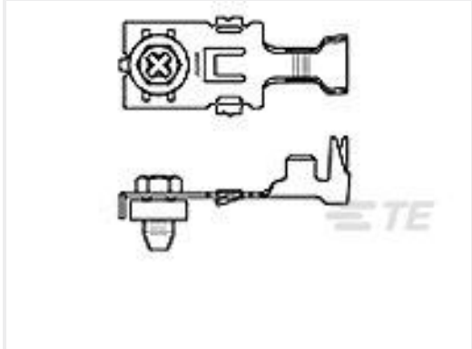
TE Part #521843-1 POWER BLOCK ASSEMBLY 16-12 AWG PTPBR
