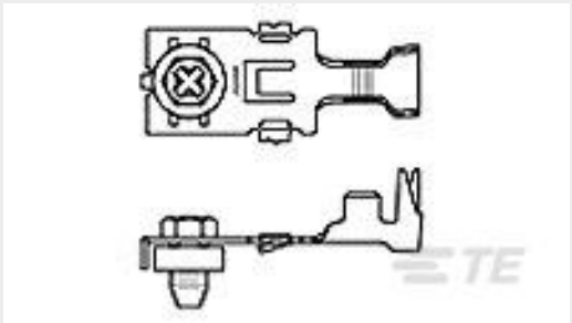
TE Part #521844-1 POWER BLOCK ASSEMBLY 16-12 AWG BR
