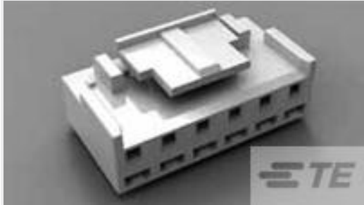
TE Part #3-1123722-6 3.96 EP PLUG HSG 6P(BLUE)
