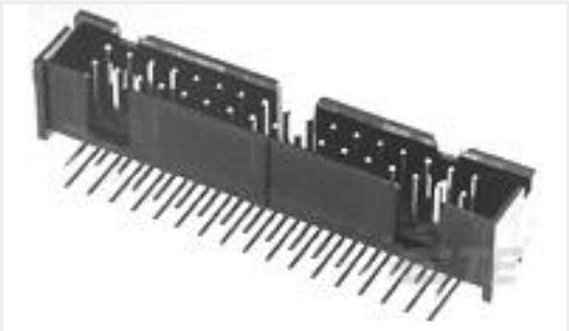
TE Part #103310-8 040 LOPRO HDR RA 15DP
