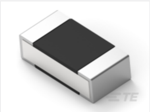
TE Part #3-2176308-9 RP 1E 0.1W 5R76 0.1% 25PPM 1K RL
