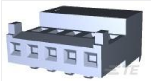
TE Part #3-644038-5 05P MTA100 CONN ASSY POL 15AU
