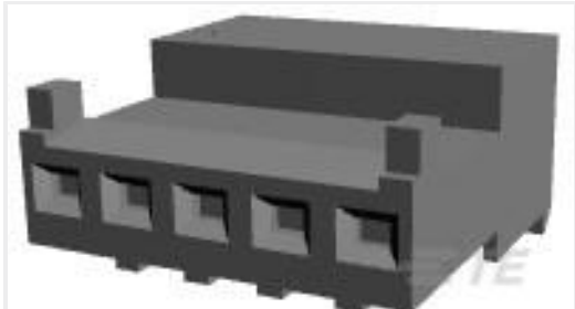
TE Part #3-643814-5 05P MTA100 CONN ASSY POL RIB
