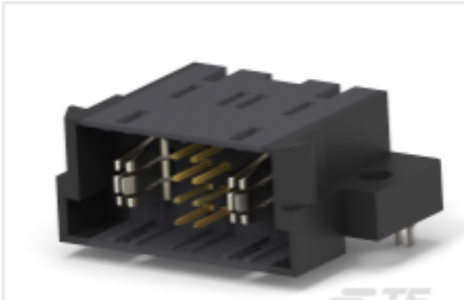
TE Part #2322144-2 MBXL R/A HDR STR 1ACP+8S+1ACP, HF
