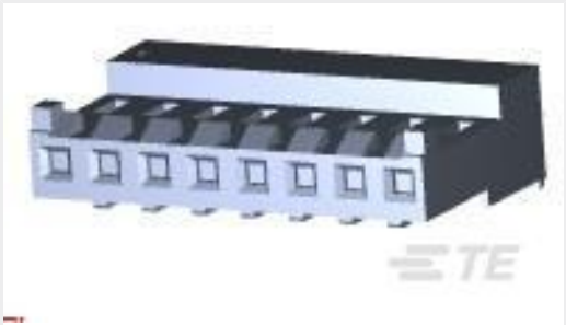
TE Part #3-643818-8 08P MTA156 CONN ASSY 20AWG YEL
