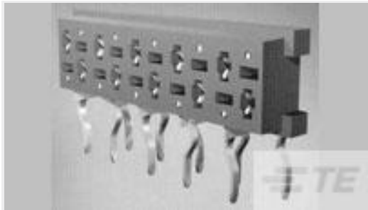
TE Part #100400-8 MICRO-MATCH FSID NP
