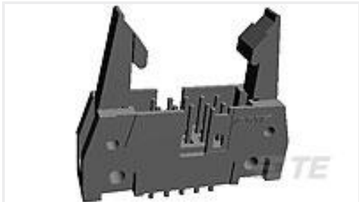
TE Part #5499910-7 A/L UNIV HDR 30P VERT SHT LAT
