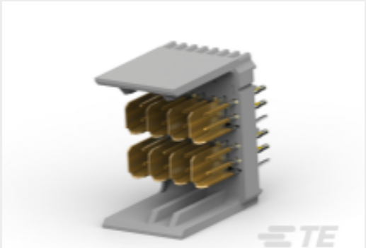
TE Part #2274678-1 HM-ZD 2PR HDR 16P 2.5MM
