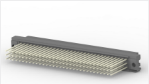
TE Part # 5536366-5 ASSY,PIN,EURO,TYPE C,LEAD-FREE, 96 POS.,.
