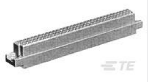
TE Part # 5536019-5 ASSY,PIN,EUROCARD,TYPE R,LEAD- FREE,96 PO
