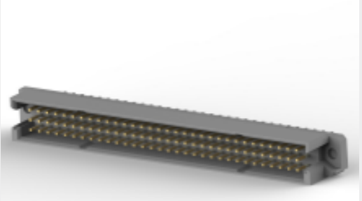
TE Part # 5535090-4 ASSEMBLY,RECEPTACLE,EUROCARD, T
