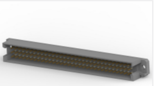
TE Part # 1-1393644-6 V42254B1100C960=PC612 MESSERLE
