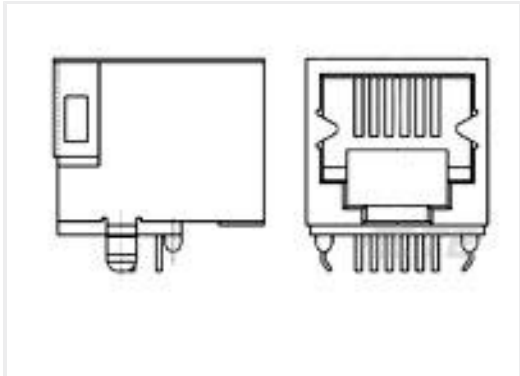
TE Part #1734723-1 RJ11,6P6C,SINGLE,DIP,W/O LED 6u"
