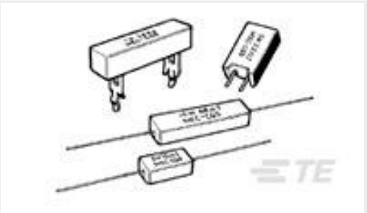
TE Part #1623785-1 SQM10 100R 5% (WIRE)
