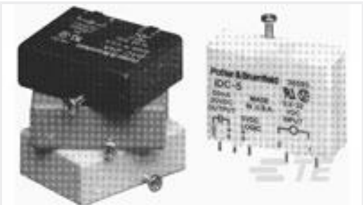
TE Part #2-1393028-5 OAC-24A = PCB MOUNT, 3A,240V AC -DC I/p
