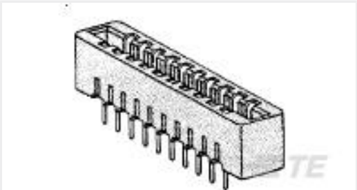
TE Part #7-530666-6 CONN LOW PRO 22 POS 156X200C/L
