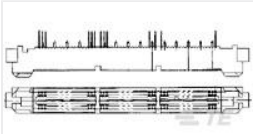
TE Part #5767039-6 MICTOR,RA PLUG,228,.093PCB,ASY
