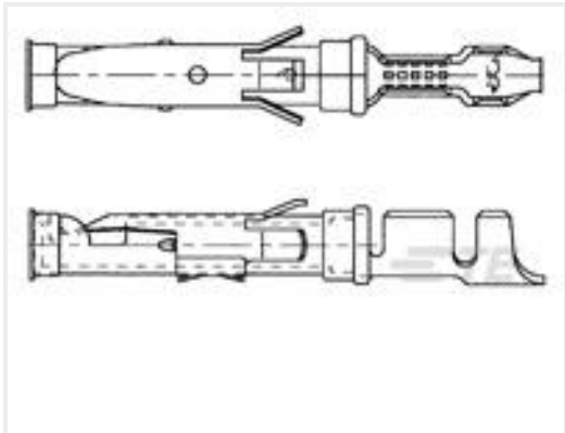
TE Part #163087-8 062 SOC.ASS. TYP3+
