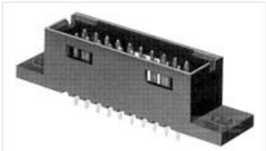
TE Part #87474-1 10 MODII HDR DRST SHRD .100CL
