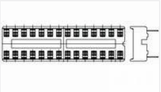
TE Part #66399-2 III+ SKT,24-20,30AU>10,LP
