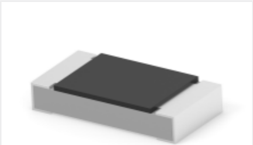
TE Part #1-2176578-3 RLC73K 2B R806 1% 5K RL
