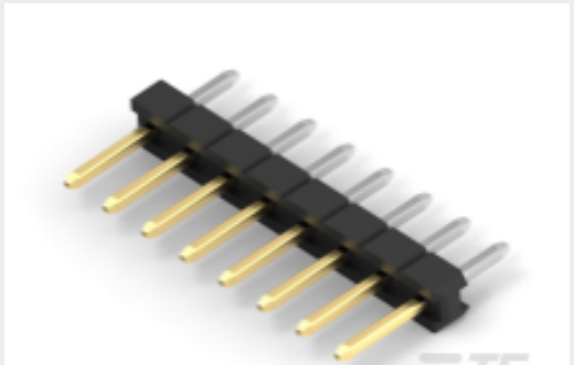
TE Part #2-2823088-5 25P,2MM,BRK HDR,SRVT,2.8,0.76AU, TB
