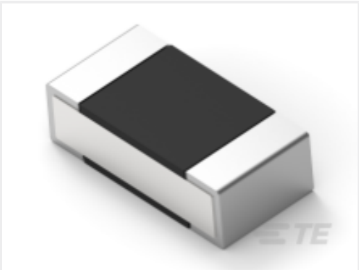
TE Part #2-2176307-1 RP 1E 0.1W 20K 0.1% 25PPM 5K RL
