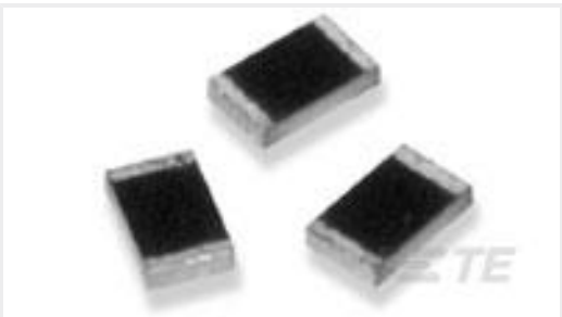
TE Part #3-1879747-7 RP 1J 150K 0.1% 15PPM CUT LENGTH
