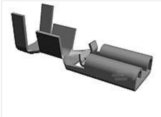
TE Part #1217114-2 187 PL MKIII REC. 18-14AWG TPBR
