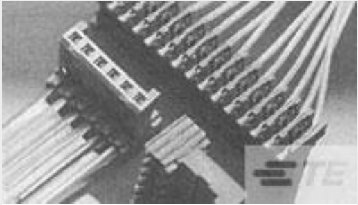
TE Part #144270-2 PLUG HE14 IDC 90 2 P AWG 24
