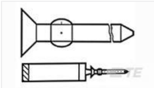
TE Part #641994-1 MTA100 KEYING PLUG W/ COD 5
