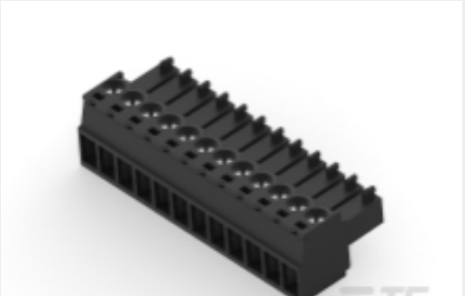
TE Part #1-2213936-2 SMT TB SCREW RECEPTACLE, 3.5 MM, 12 POS
