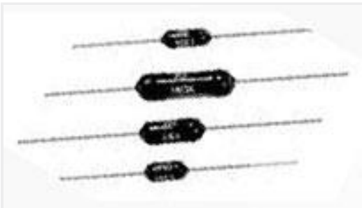
TE Part #1-1879666-8 H8 200K 0.1% 15PPM
