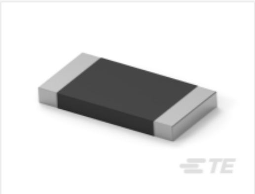
TE Part #6-2176421-0 TLRP 2512 2.0W R040 1% 50PPM 4K RL
