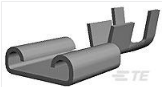
TE Part #5-160465-1 250 FASTON REC 18-16 AWG BR
