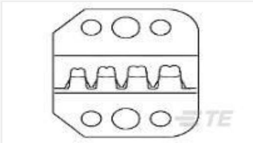
TE Part #90546-2 PROCrimper Die Assy Univ MNL
