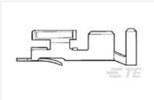
TE Part #350650-1 HCC 12-18 025PTPHBZ,LUBED
