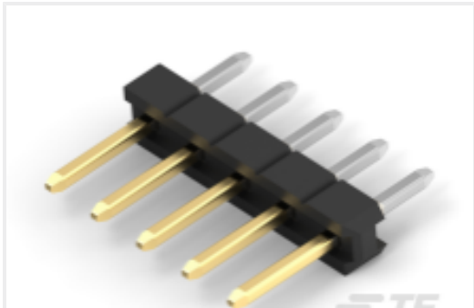
TE Part #2355186-6 6P,2MM,BRK HDR,SRVT,2.8,0.76AU, BOX
