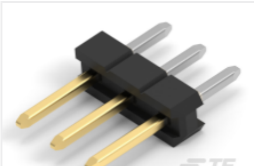
TE Part #2355186-3 3P,2MM,BRK HDR,SRVT,2.8,0.76AU, BOX
