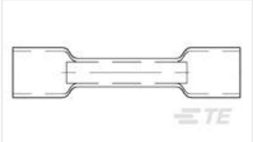
TE Part #603504-2 12-10 PRE-INSUL SEALED SPLICE
