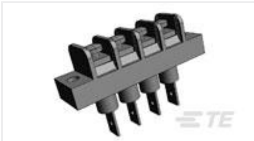
TE Part #5-1437665-3 JC6-Q307-04=JC6 ASSEMBLY
