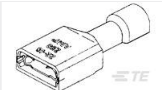
TE Part #3-520404-2 ULTRA-FAST 187 ASY REC 16-14 AWG TPBR
