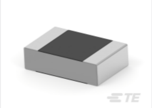
TE Part #2176238-3 CPF A 0805 13R3 0.1% 25PPM 5K RL
