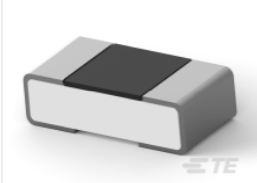
TE Part #6-2176363-8 RQ 0402 2K15 0.1% 10PPM 5K RL
