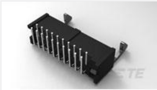
TE Part #2-1761607-7 IDC LOW PRO HDR 20P RA LAT
