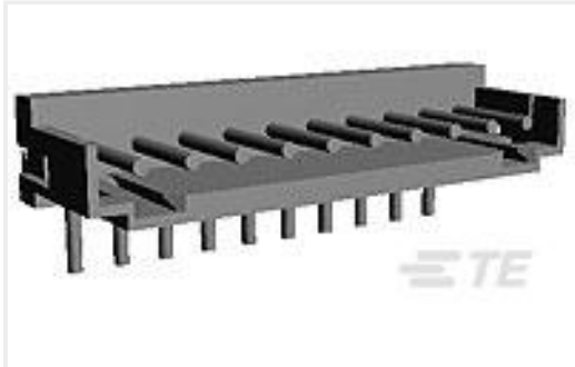
TE Part #292253-3 CT CONN MT HDR ASSY H 3P NAT
