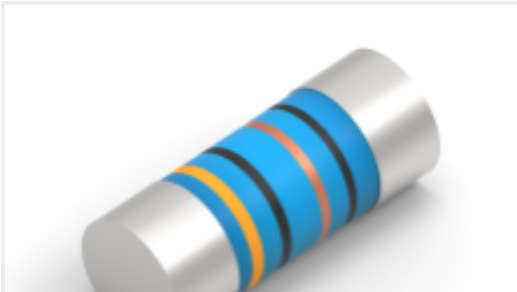
TE Part #8-2176315-1 MELF SMA-A 33R 1% 50PPM 0204 0.4 W
