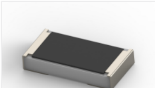
TE Part #2176469-2 TLRP 2010 2.0W R020 1% 75PPM 4K RL
