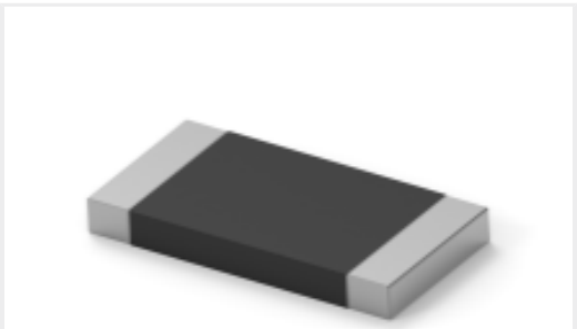
TE Part #2-2176422-8 TLRP 2512 3.0W R035 1% 25PPM 4K RL
