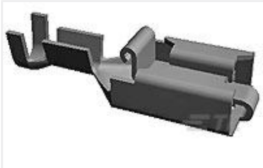
TE Part #170234-2 PL 250 REC 12-10 AWG 0.406 X 42.3
