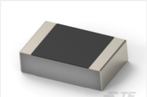
TE Part #7-2176452-1 CPF 0201 2K87 0.1% 25ppm 1K RL
