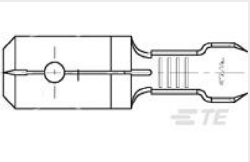
TE Part #626377-1 TERMINAL FASTON .250 TAB 22-18 AWG BR
