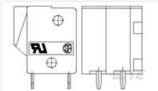
TE Part #1776260-3 3P Spring TB, 180deg, VT,5.08mm, Green
