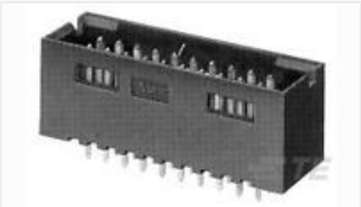
TE Part #5-103169-4 12 MODII HDR DRST SHRD .100CL
